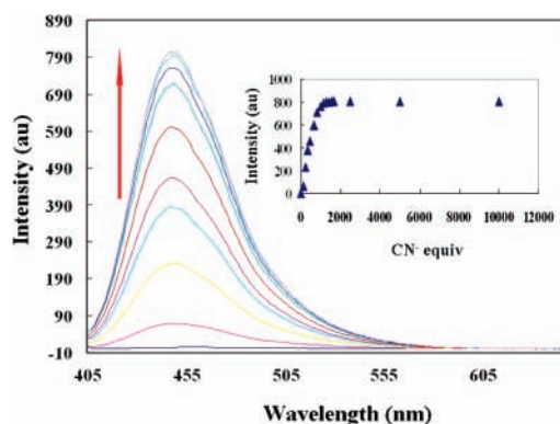
Figure 2. Fluorescence titration spectra of the dosimeter upon addition of cyanide anion. Inset: Fluorescence change of the sensor against [CN^-]/[I] ( [I] = 10 \mu M , \lambda_{ex} = 360 nm, \lambda_{em} = 450 nm).
