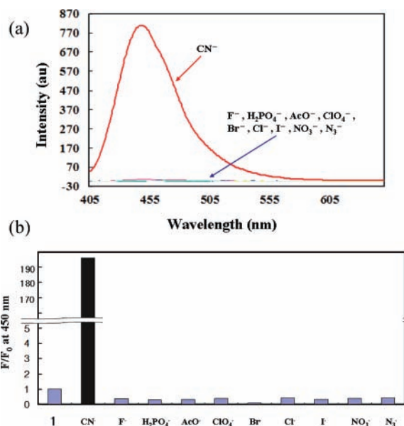
Figure 3. (a) Fluorescence spectra of the dosimeter (10 \mu M) in HEPES upon addition of 1500 equiv of various anions (from left to right: only the sensor, CN^- , F^- , H_2PO_4^- , AcO^- , ClO_4^- , Br^- , Cl^- , I^- , NO_3^- , N_3^- ) (sodium salts). (b) Its relative fluorescence intensities.
