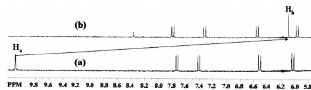
Figure 1. ^1H NMR spectral change of the dosimeter upon addition of cyanide anions: (a) sensor only and (b) sensor and 10 equiv of NaCN ( [I] = 10 mM in D_2O at 25 °C).
